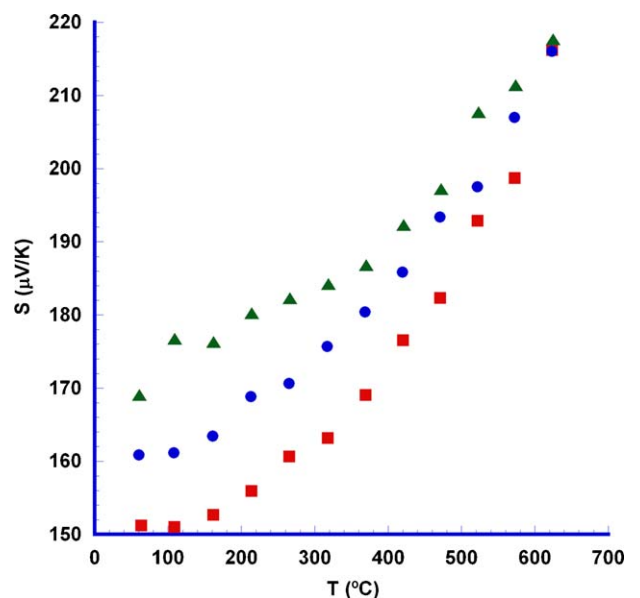
Fig. 7. Temperature dependence of the thermopower of \text{Bi}_2\text{Ca}_2\text{Co}_{1.7}\text{O}_x for each type of sample. (■) solid state; (●) sol-gel; and (▲) polymer solution.
