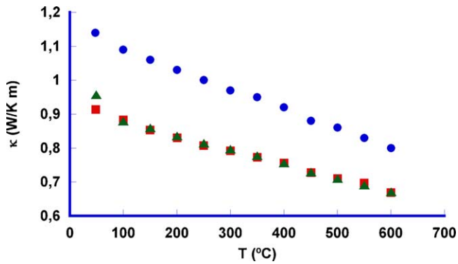
Fig. 8. Temperature dependence of the thermal conductivity of \text{Bi}_2\text{Ca}_2\text{Co}_{1.7}\text{O}_x for each type of sample. (■) solid state; (●) sol-gel; and (▲) polymer solution.
