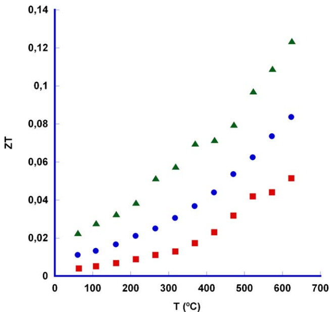
Fig. 9. Temperature dependence of ZT for the \text{Bi}_2\text{Ca}_2\text{Co}_{1.7}\text{O}_x samples prepared by the different synthetic methods. (■) solid state; (●) sol-gel; and (▲) polymer solution.
