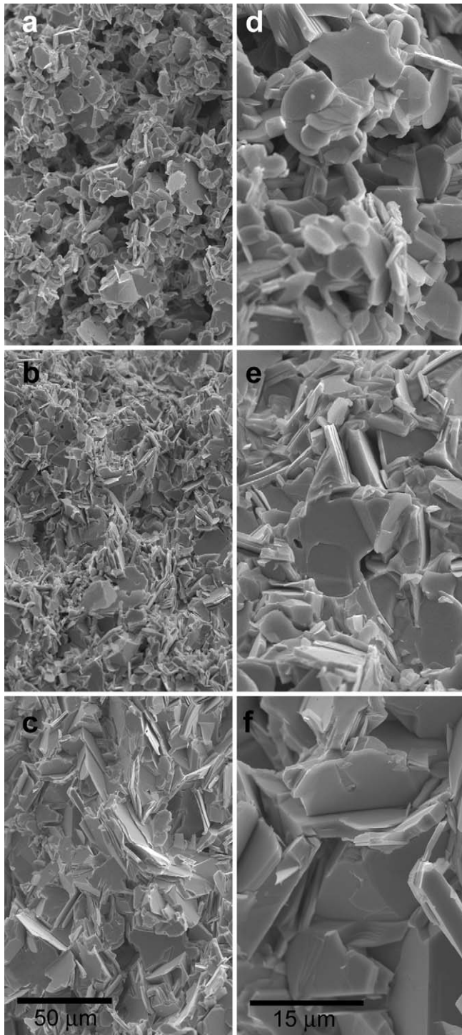
Fig. 4. Scanning electron micrographs from transversal fractured samples \text{Bi}_2\text{Ca}_2\text{Co}_{1.7}\text{O}_x obtained by solid-state (a and d), sol-gel (b and e), and polymer (c and f) reaction methods.
