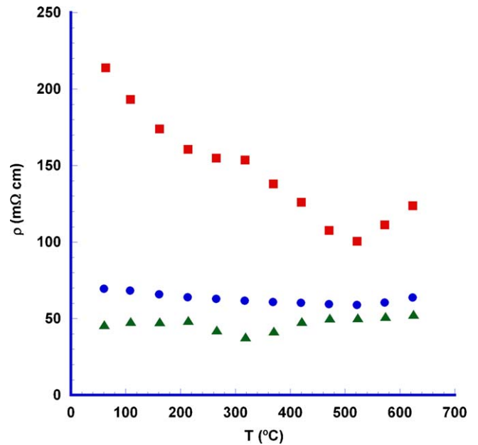
Fig. 6. Temperature dependence of the electrical resistivity of \text{Bi}_2\text{Ca}_2\text{Co}_{1.7}\text{O}_x for each type of sample. (■) solid state; (●) sol-gel; and (▲) polymer solution.
