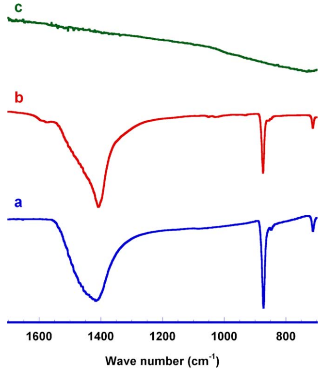
Fig. 2. FTIR curves obtained, in ATR mode, in different steps of the synthetic procedure: after burning the dry products from the (a) sol-gel and (b) polymer solution method. Curve (c) shows the spectra of the polymer sample after thermal treatment at 750 °C for 12 h.
