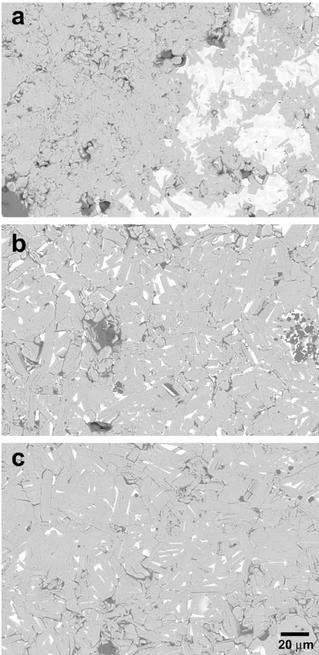
Fig. 5. Scanning electron micrographs from longitudinal polished samples \text{Bi}_2\text{Ca}_2\text{Co}_{1.7}\text{O}_x obtained by solid-state (a), sol-gel (b), and polymer (c) reaction methods.
