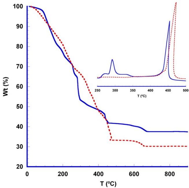
Fig. 1. TGA plot vs. temperature of the initial solutions (—) sol-gel and (---) polymer solution methods. The insert shows the DTA curve in the coordination compounds decomposition temperature range.
