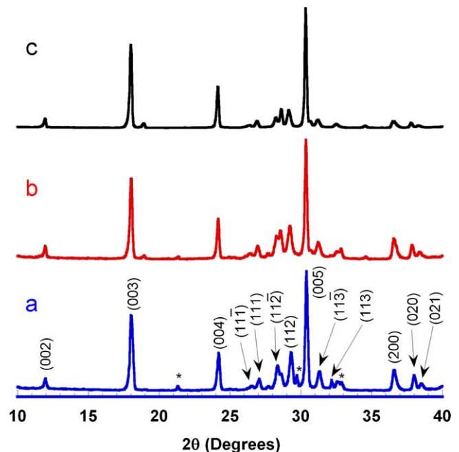
Fig. 3. XRD plots of the \text{Bi}_2\text{Ca}_2\text{Co}_{1.7}\text{O}_x sintered specimens obtained for the different synthetic methods. (a) Solid state, (b) sol-gel, and (c) polymer solution.
